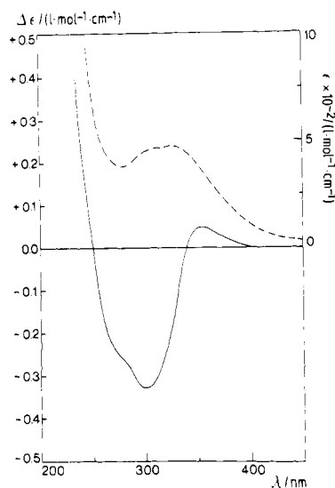
Figure 4. CD (—) and UV (---) spectra of polymer 3h in n -hexane solution.
